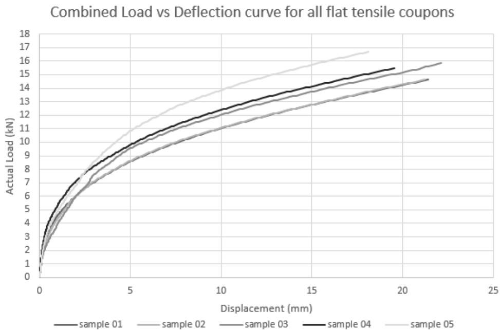
Figure 04: Combined load vs deflection curve for all flat tensile coupons
