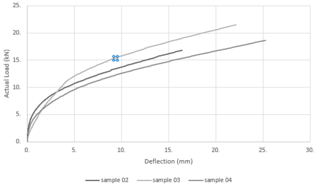
Figure 05: Combined load vs deflection curve for all overlap splice tensile coupons
