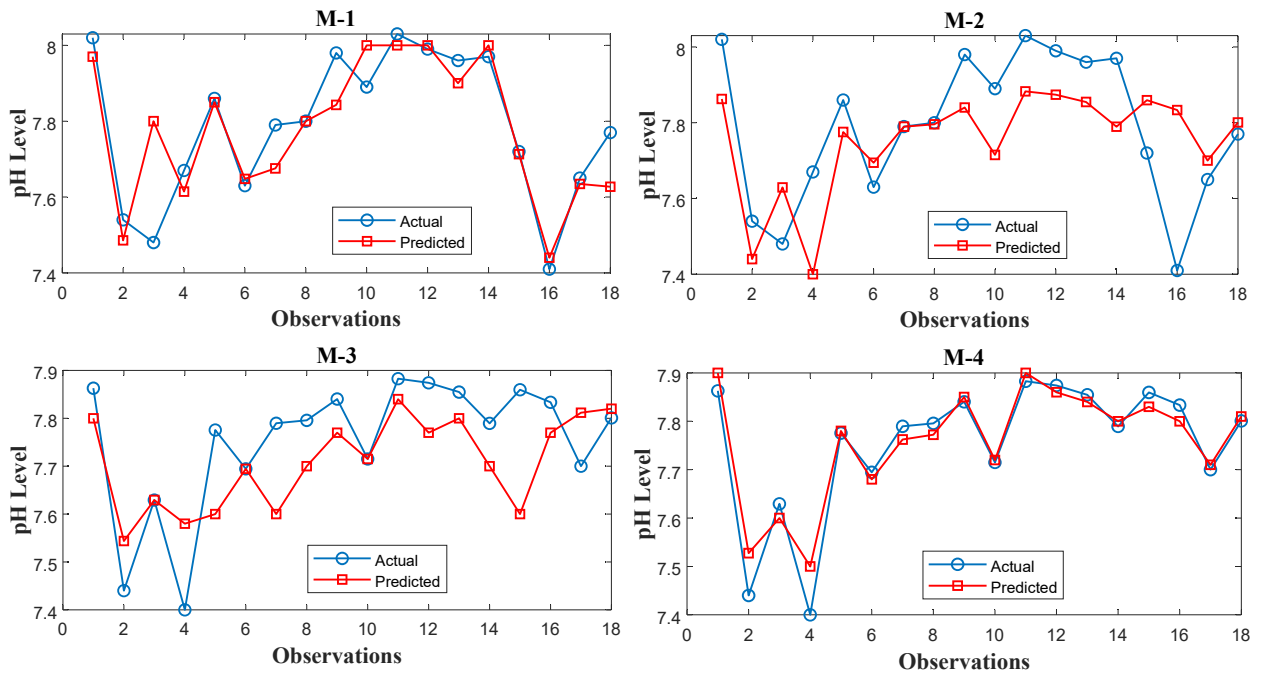
Figure 5: Forecast Results of the M-1, M-2, M-3, and M-4 Models
