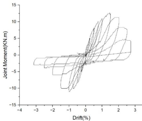
Fig. 4.3: Joint moment vs drift ratio curve for SP-3
