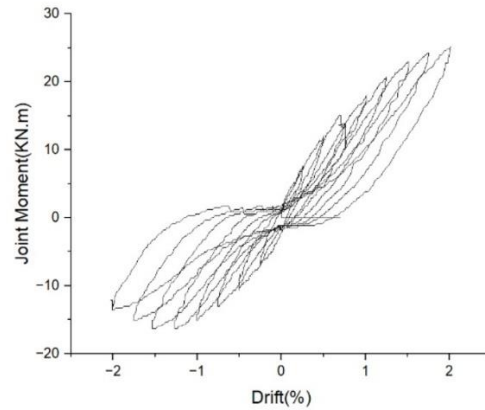
Fig. 4.2: Joint moment vs drift ratio curve for SP-2
