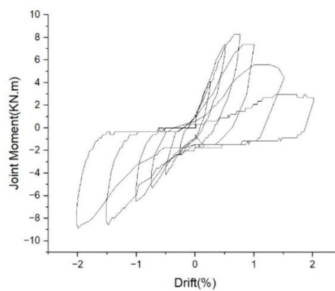
Fig.4.4: Joint moment vs drift ratio curve for SP-4
