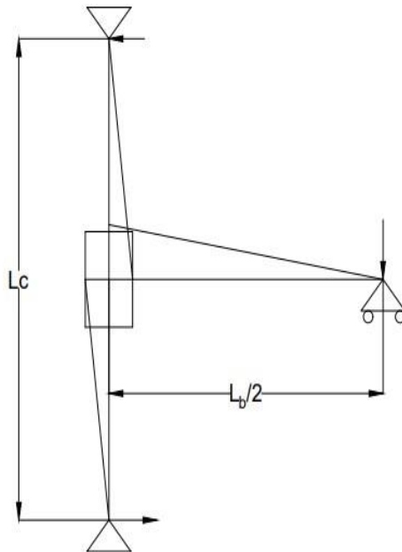
Fig. 3.1: Seismic moment diagram
