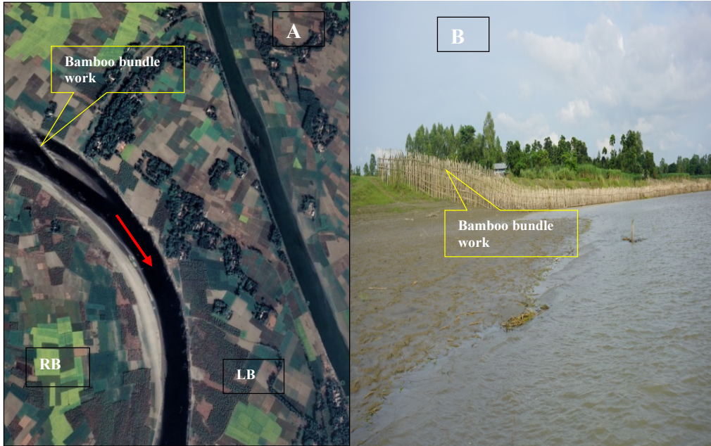
Figure 8: Picture (A) planform view of bamboo bundle work Google image 2018 work and picture (B) field image of bamboo bundle work along left bank of Old Brahmaputra River.
