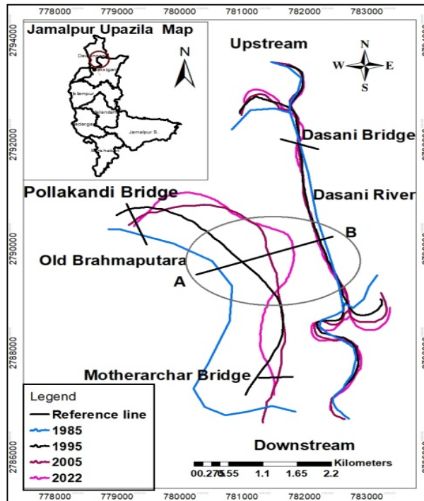
Figure 9: Plan form change of Old Brahmaputra and Dasani at study area during 1985 to 2022.
