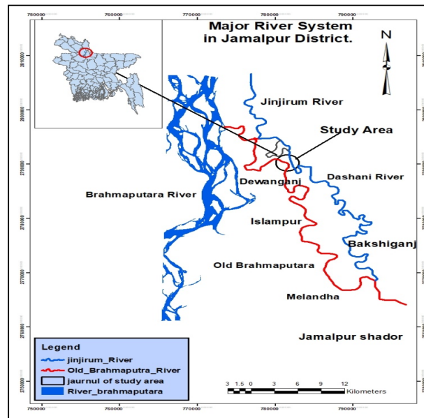
Figure 1: Planform of the rivers system in Jamalpur district (Google image 2023).
