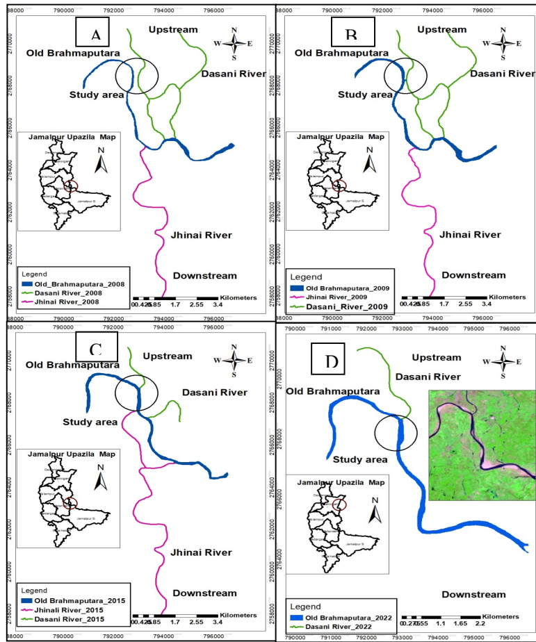
Figure 5: Plan form change Old Brahmaputra and Dasani Rivers near at Jamalpur Sadar during the years 2008(A), 2009(B), 2015(C) and 2022(D)
