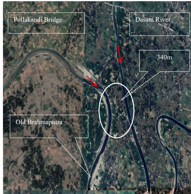
Figure 2: Plan form of rivers near at Modonairchara Baksiganj in Jamalpur district (Google image 17/11/2022)
