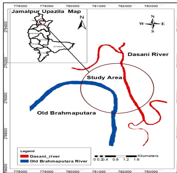
Figure 3: Study area showing Old Brahmaputra River and Dasani River
