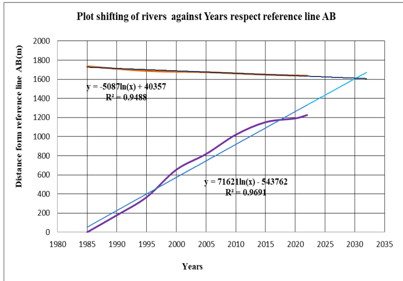
Figure 11: Graph plot for shifting of rivers against years respect with reference line AB.
